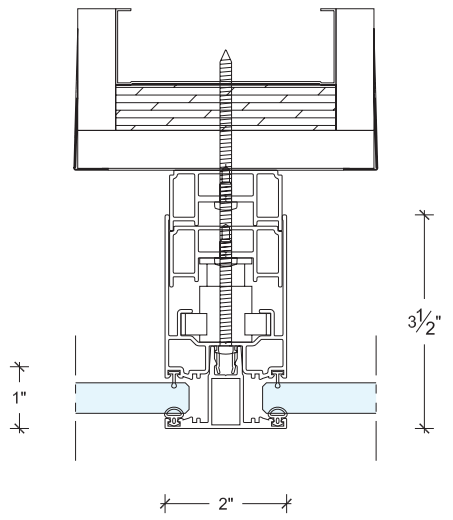
FLYBY WITH SINGLE GLAZED FLYBY EN VERRE SIMPLE
