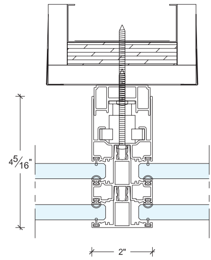
FLYBY WITH DOUBLE GLAZED FLYBY EN VERRE DOUBLE
